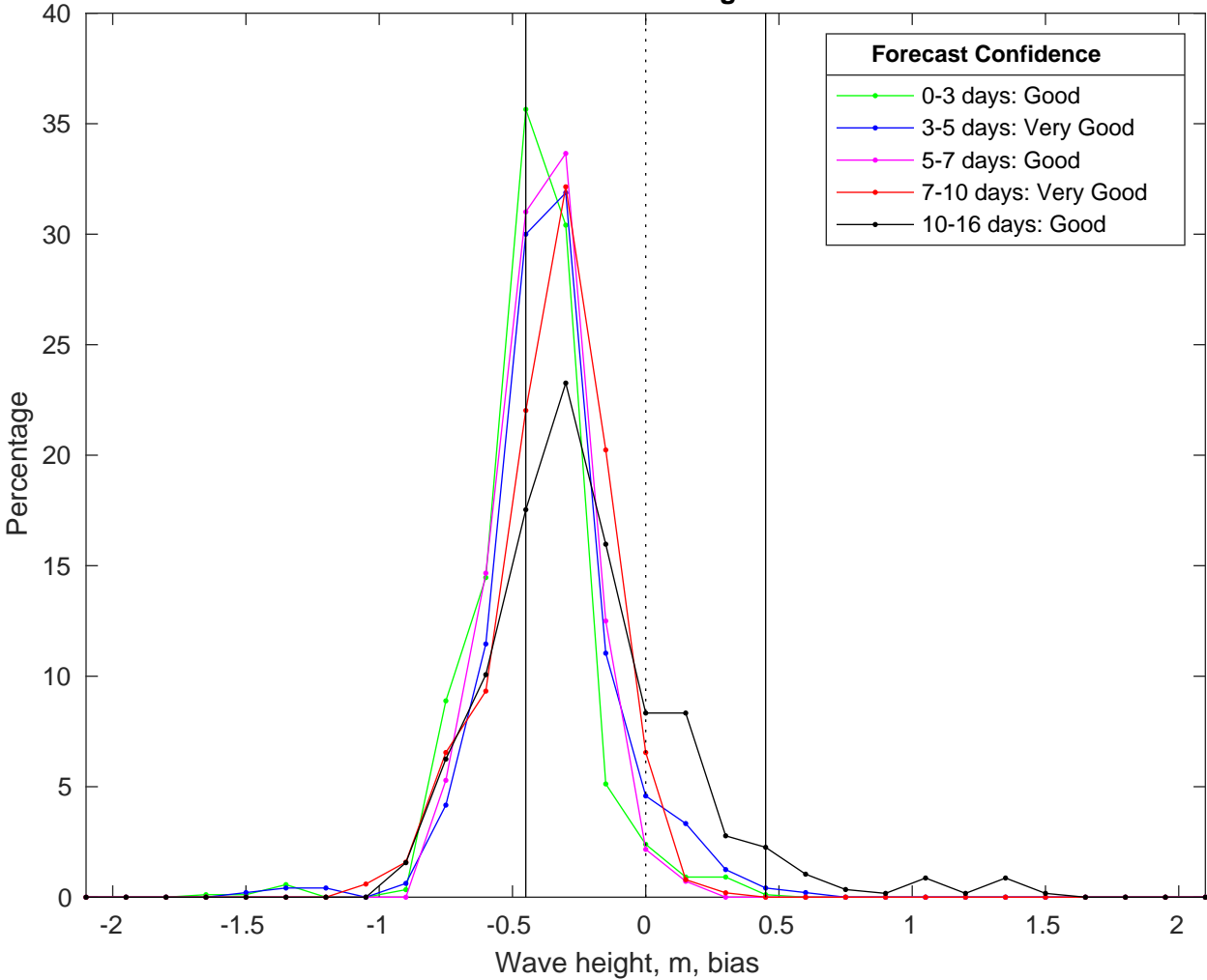
NDBC 52213 vs GFS Waves Bias Histogram: 31-Jul-2025
