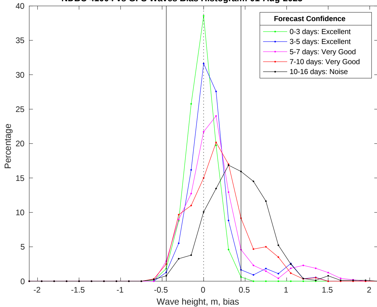
NDBC 41004 vs GFS Waves Bias Histogram: 01-Aug-2025
