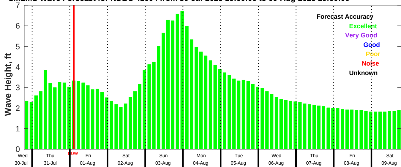
CMEMS Wave Forecast for NDBC 41004 from 30-Jul-2025 19:00:00 to 09-Aug-2025 19:00:00
