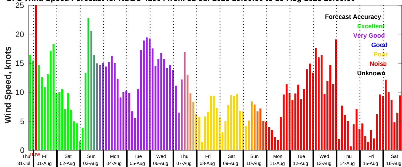
GFS Wind Speed Forecast for NDBC 41004 from 31-Jul-2025 19:00:00 to 16-Aug-2025 19:00:00
