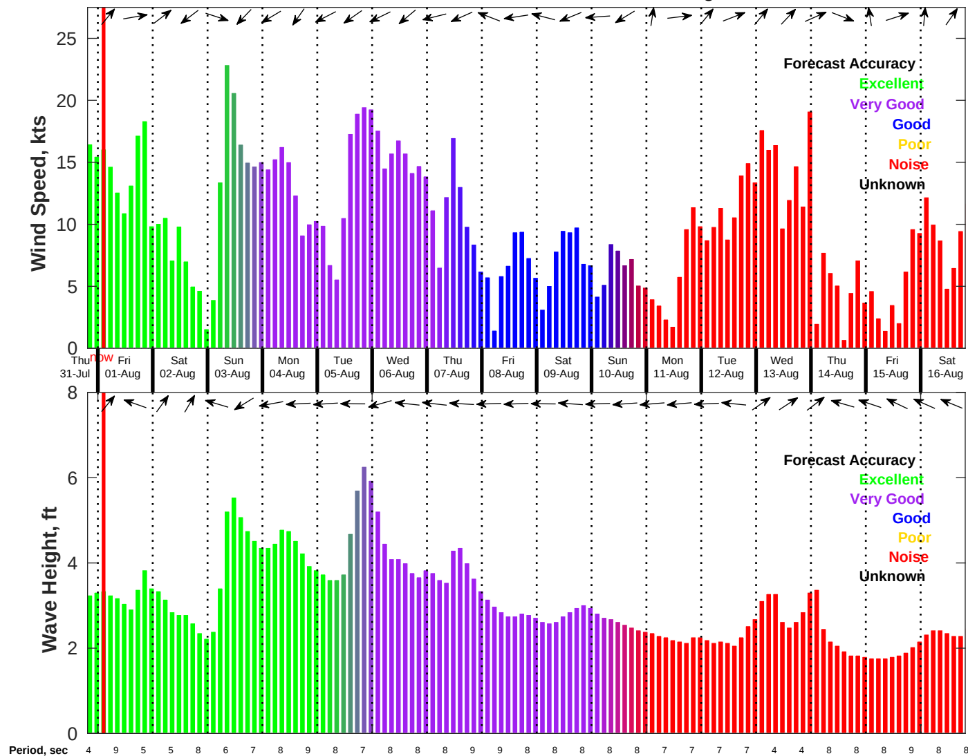
Wind & Wave Forecast for NDBC 41004 from 31-Jul-2025 19:00:00 to 16-Aug-2025 19:00:00
