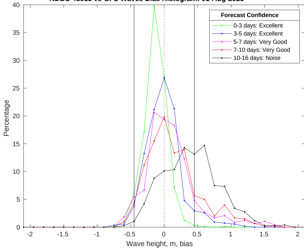
NDBC 41013 vs GFS Waves Bias Histogram: 01-Aug-2025
