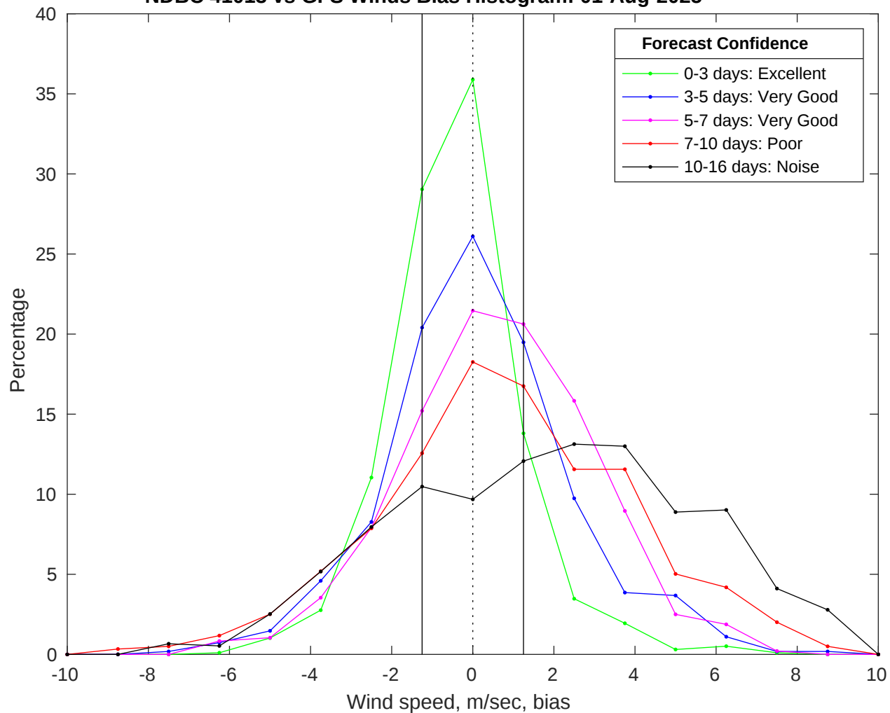
NDBC 41013 vs GFS Winds Bias Histogram: 01-Aug-2025
