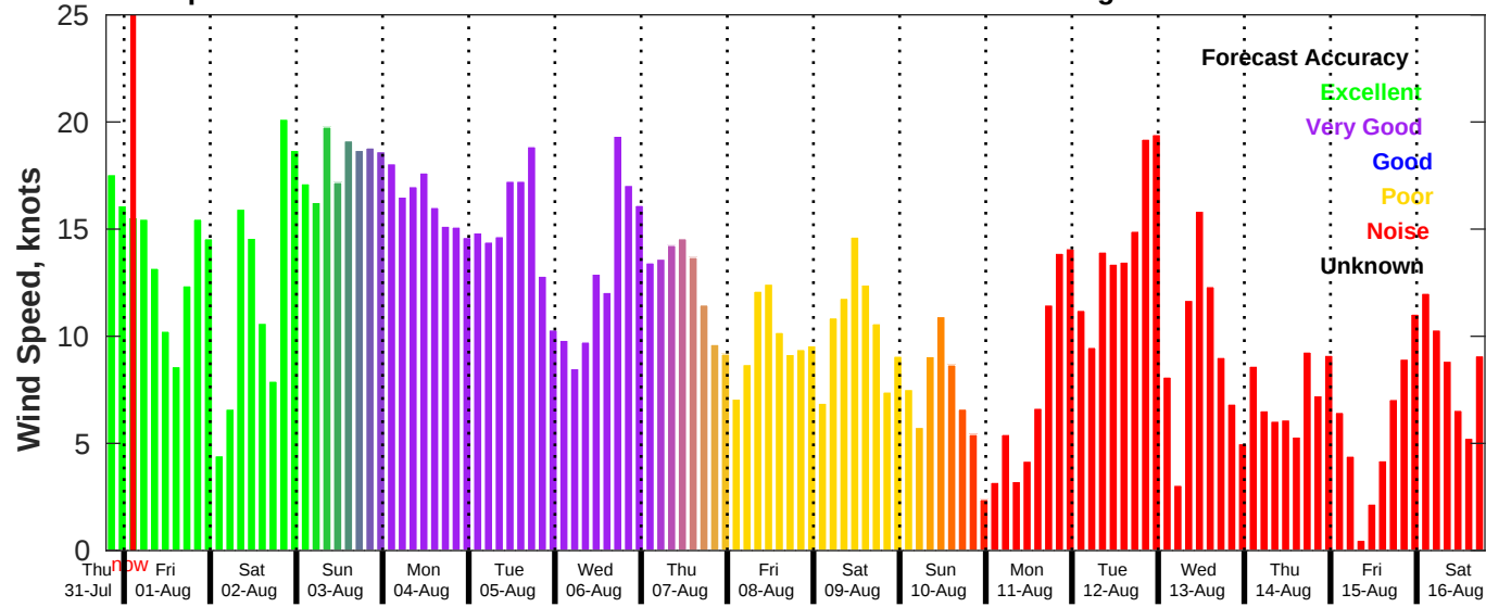
GFS Wind Speed Forecast for NDBC 41013 from 31-Jul-2025 19:00:00 to 16-Aug-2025 19:00:00
