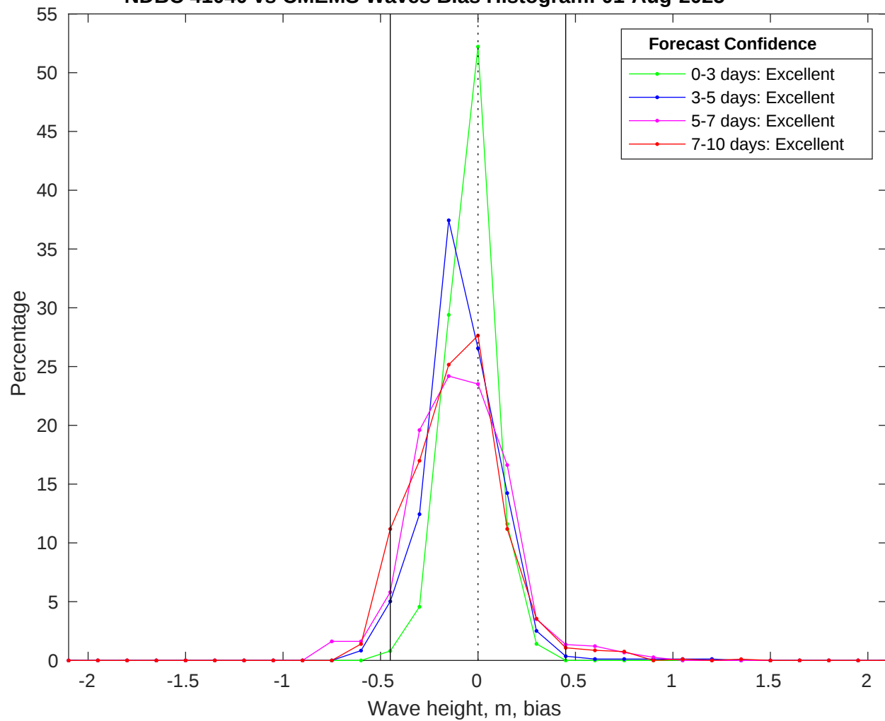
NDBC 41040 vs CMEMS Waves Bias Histogram: 01-Aug-2025
