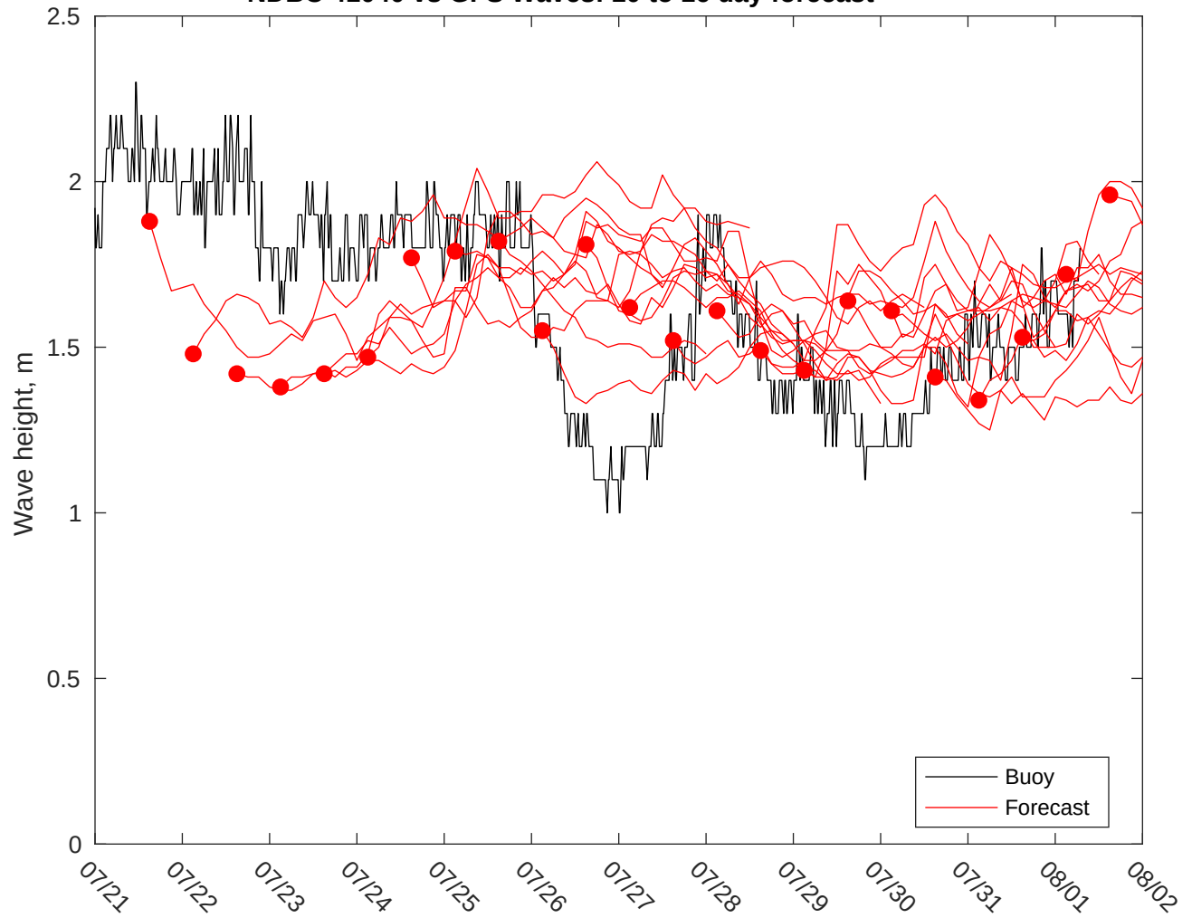
NDBC 41040 vs GFS Waves: 10 to 16 day forecast
