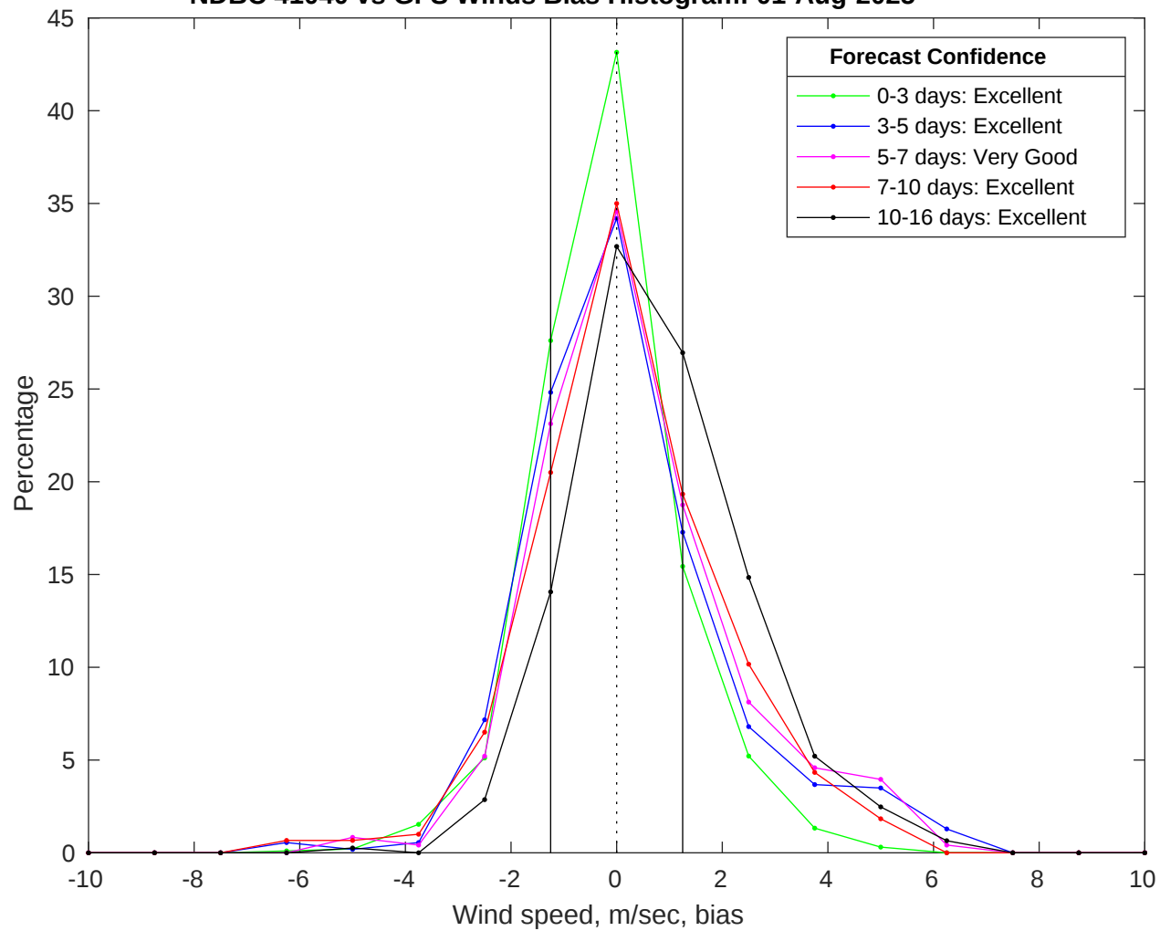
NDBC 41040 vs GFS Winds Bias Histogram: 01-Aug-2025
