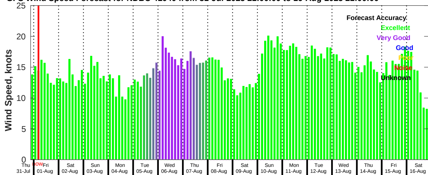
GFS Wind Speed Forecast for NDBC 41040 from 31-Jul-2025 21:00:00 to 16-Aug-2025 21:00:00
