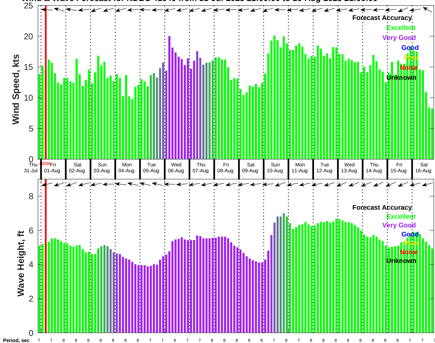
Wind & Wave Forecast for NDBC 41040 from 31-Jul-2025 21:00:00 to 16-Aug-2025 21:00:00
