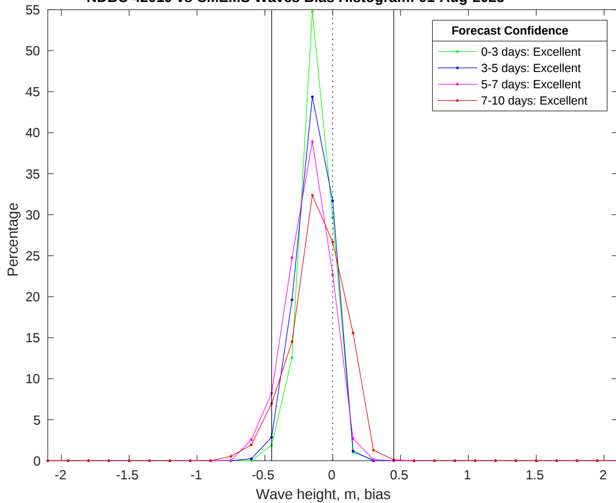
NDBC 42019 vs CMEMS Waves Bias Histogram: 01-Aug-2025
