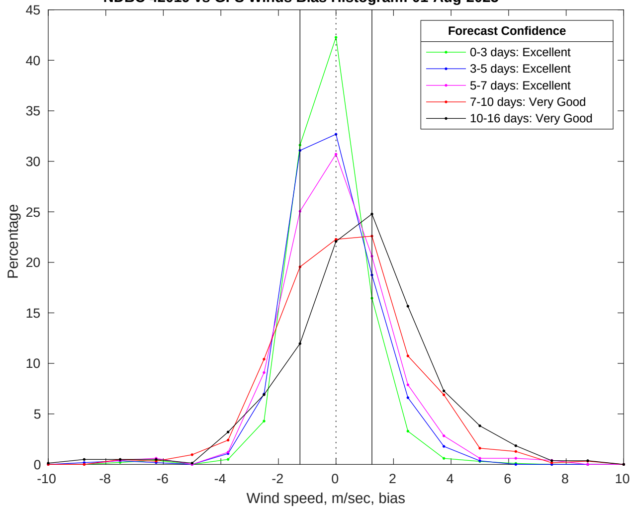
NDBC 42019 vs GFS Winds Bias Histogram: 01-Aug-2025
