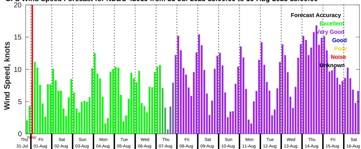
GFS Wind Speed Forecast for NDBC 42019 from 31-Jul-2025 18:00:00 to 16-Aug-2025 18:00:00
