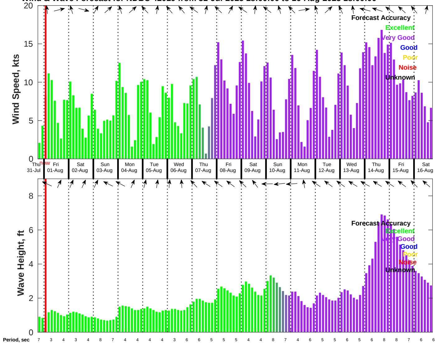
Wind & Wave Forecast for NDBC 42019 from 31-Jul-2025 18:00:00 to 16-Aug-2025 18:00:00
