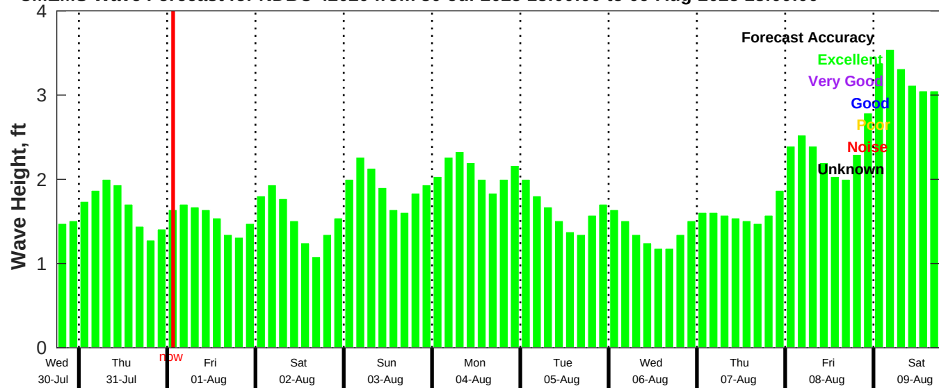
CMEMS Wave Forecast for NDBC 42020 from 30-Jul-2025 18:00:00 to 09-Aug-2025 18:00:00
