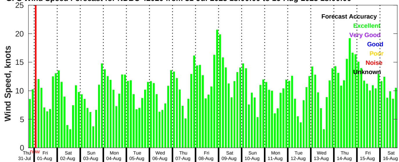
GFS Wind Speed Forecast for NDBC 42020 from 31-Jul-2025 18:00:00 to 16-Aug-2025 18:00:00
