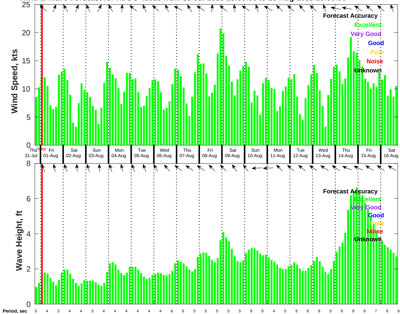
Wind & Wave Forecast for NDBC 42020 from 31-Jul-2025 18:00:00 to 16-Aug-2025 18:00:00
