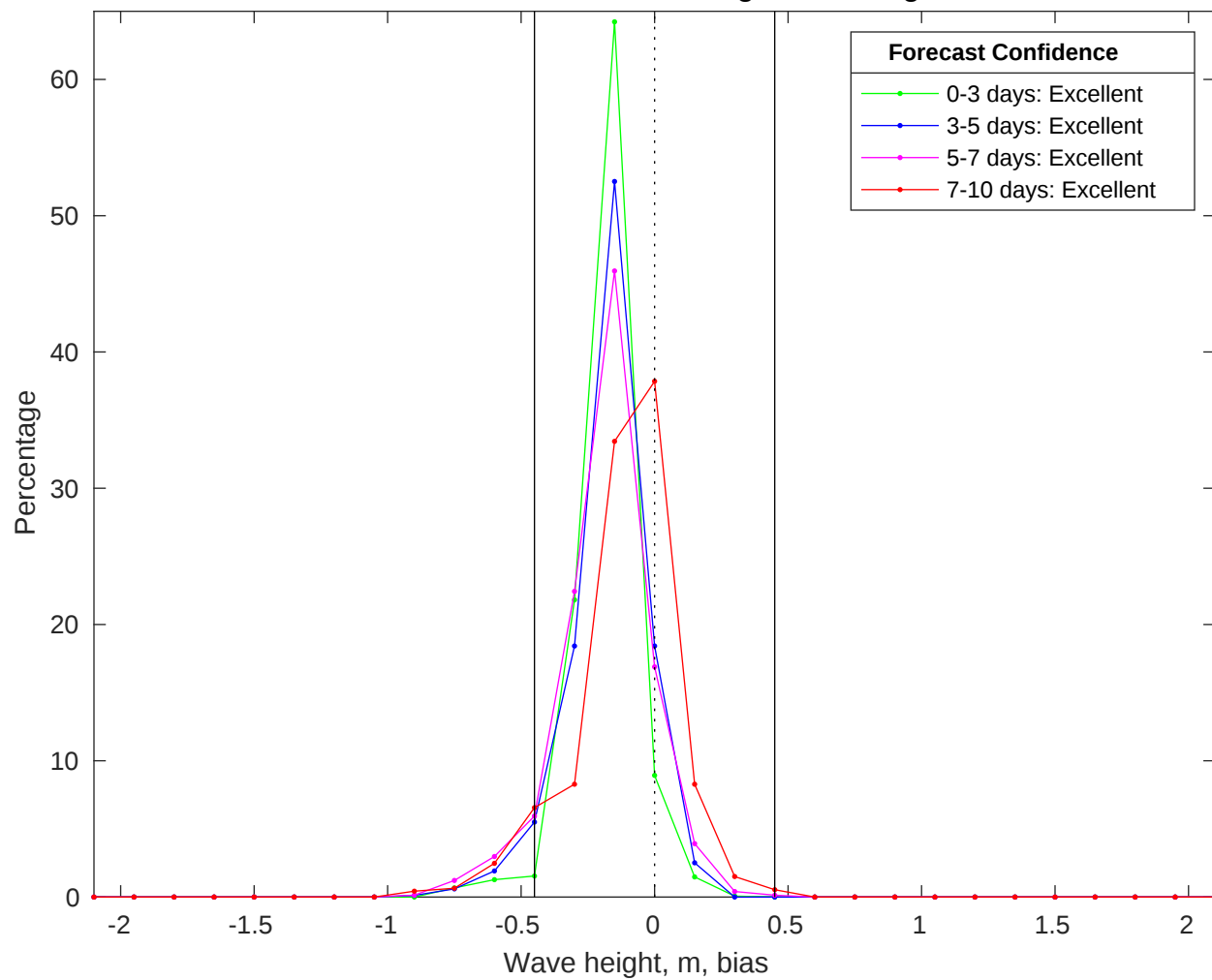
NDBC 42035 vs CMEMS Waves Bias Histogram: 01-Aug-2025
