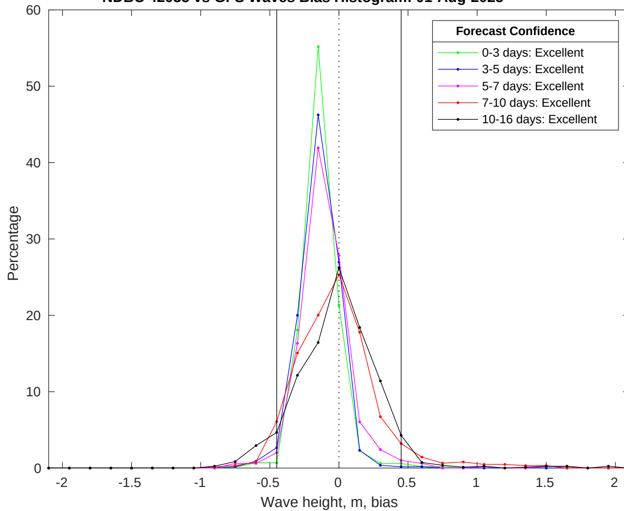
NDBC 42035 vs GFS Waves Bias Histogram: 01-Aug-2025
