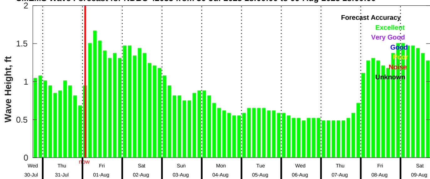
CMEMS Wave Forecast for NDBC 42035 from 30-Jul-2025 18:00:00 to 09-Aug-2025 18:00:00
