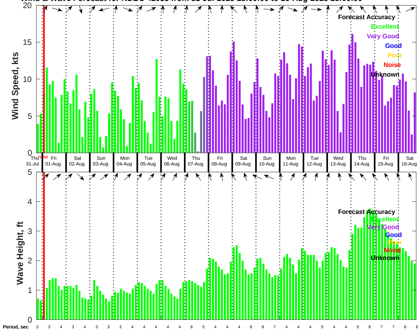
Wind & Wave Forecast for NDBC 42035 from 31-Jul-2025 18:00:00 to 16-Aug-2025 18:00:00
