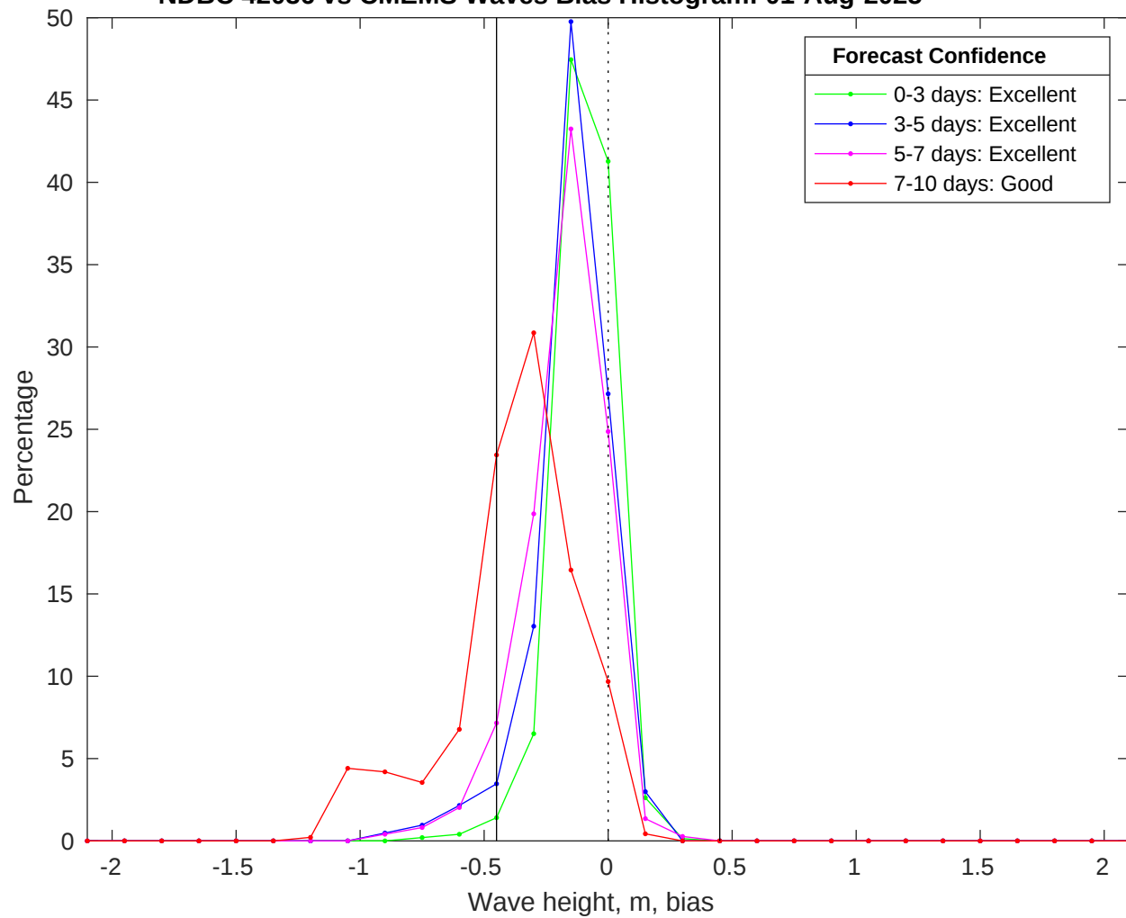
NDBC 42036 vs CMEMS Waves Bias Histogram: 01-Aug-2025
