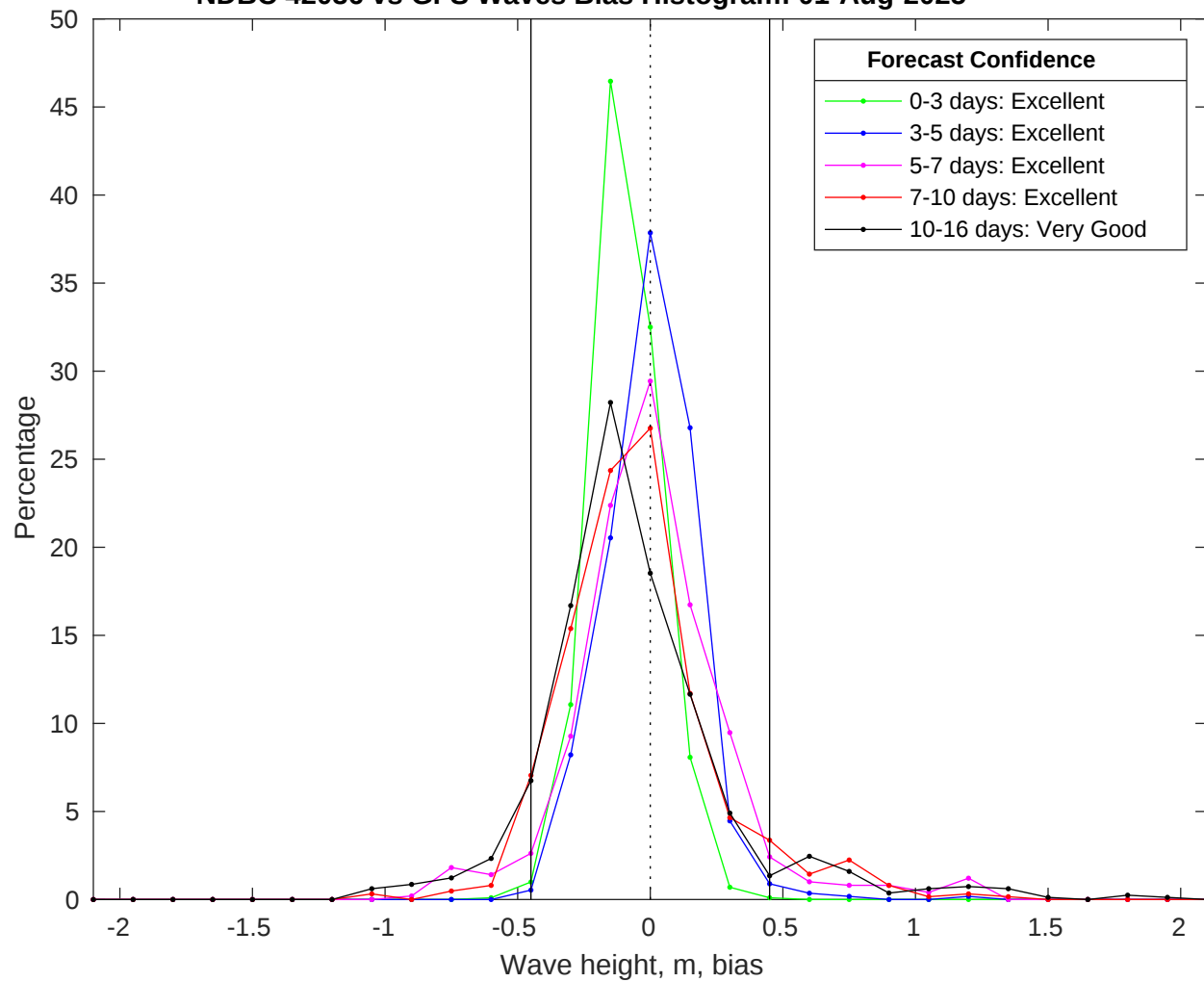
NDBC 42036 vs GFS Waves Bias Histogram: 01-Aug-2025
