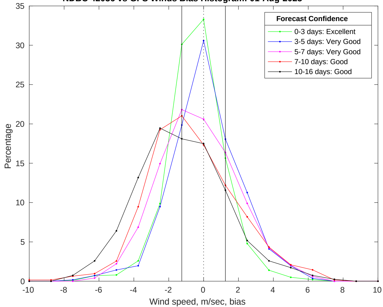
NDBC 42036 vs GFS Winds Bias Histogram: 01-Aug-2025
