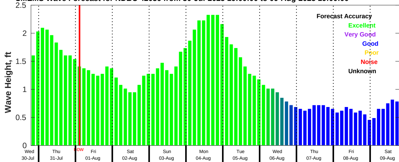
CMEMS Wave Forecast for NDBC 42036 from 30-Jul-2025 19:00:00 to 09-Aug-2025 19:00:00
