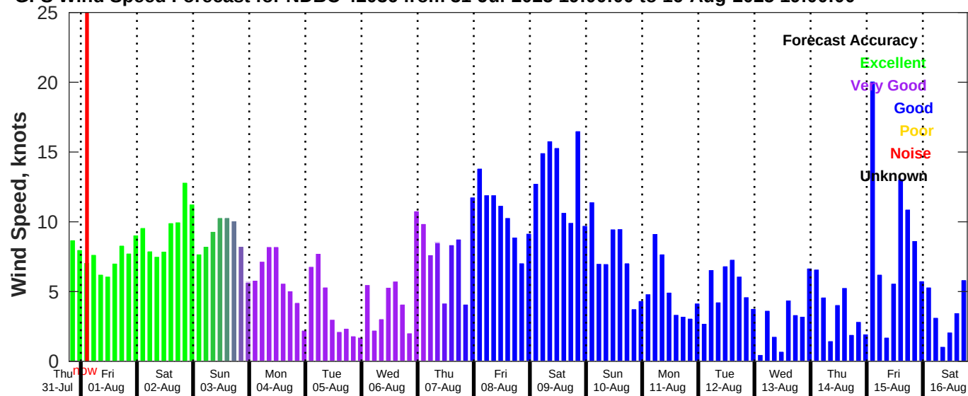
GFS Wind Speed Forecast for NDBC 42036 from 31-Jul-2025 19:00:00 to 16-Aug-2025 19:00:00
