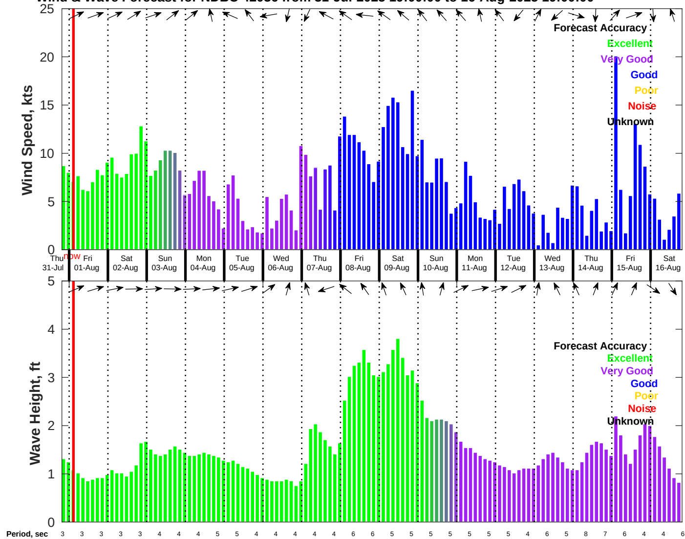
Wind & Wave Forecast for NDBC 42036 from 31-Jul-2025 19:00:00 to 16-Aug-2025 19:00:00
