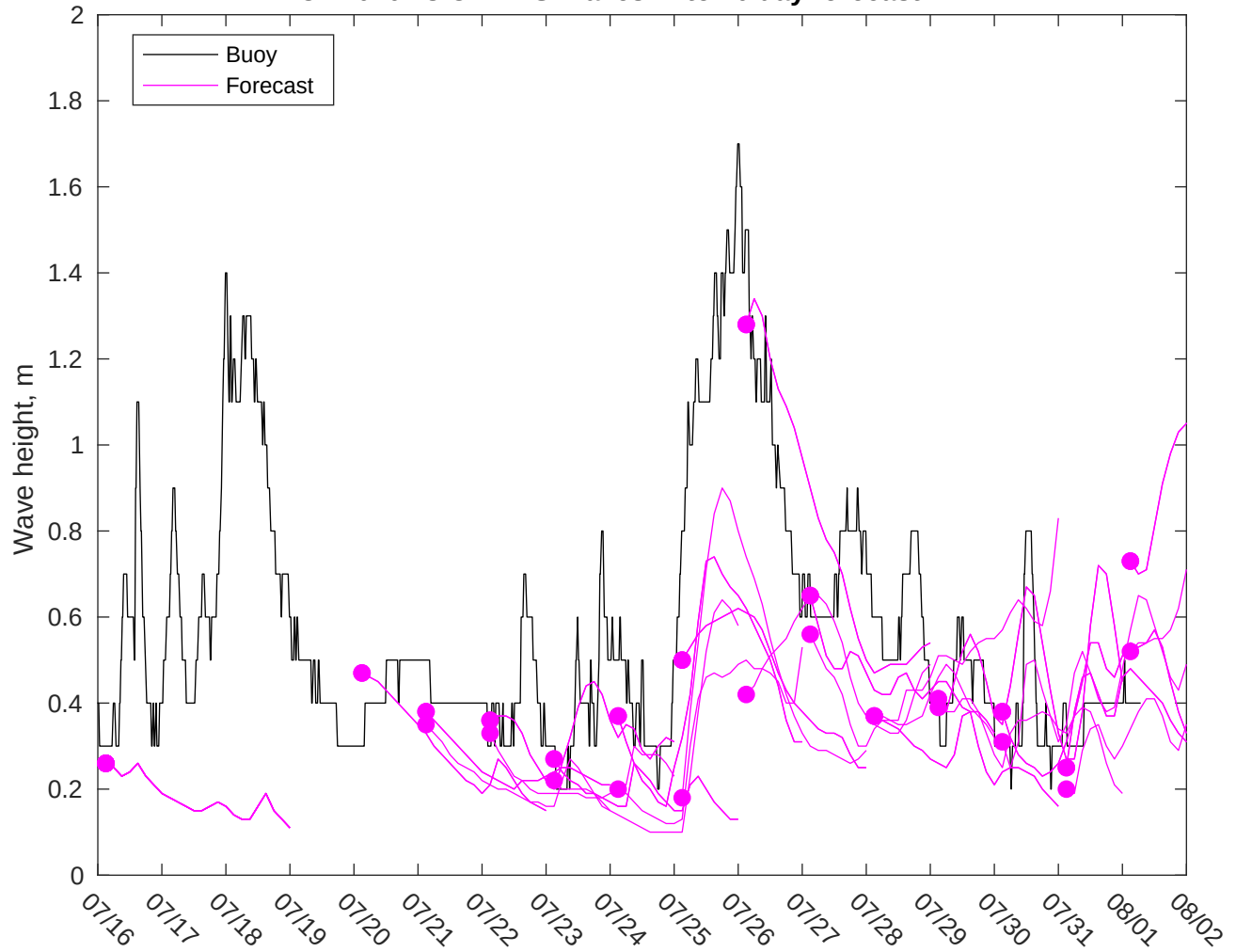
NDBC 42040 vs CMEMS Waves: 7 to 10 day forecast
