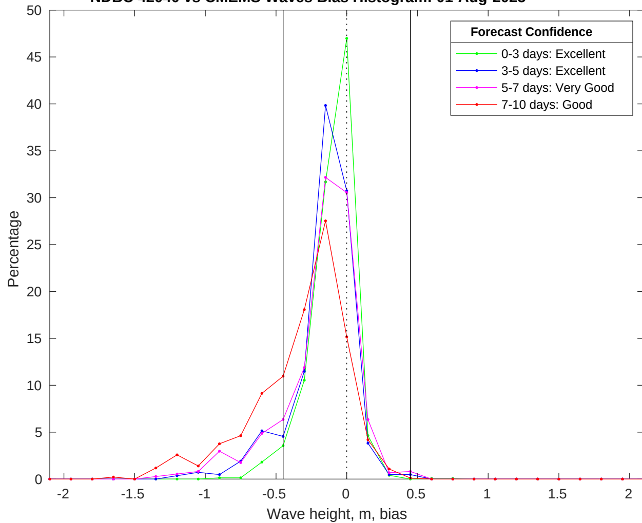
NDBC 42040 vs CMEMS Waves Bias Histogram: 01-Aug-2025
