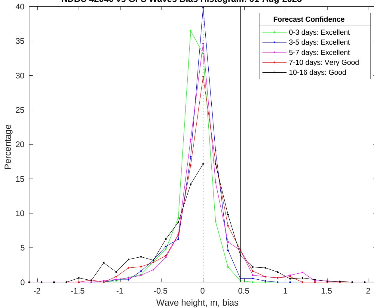
NDBC 42040 vs GFS Waves Bias Histogram: 01-Aug-2025
