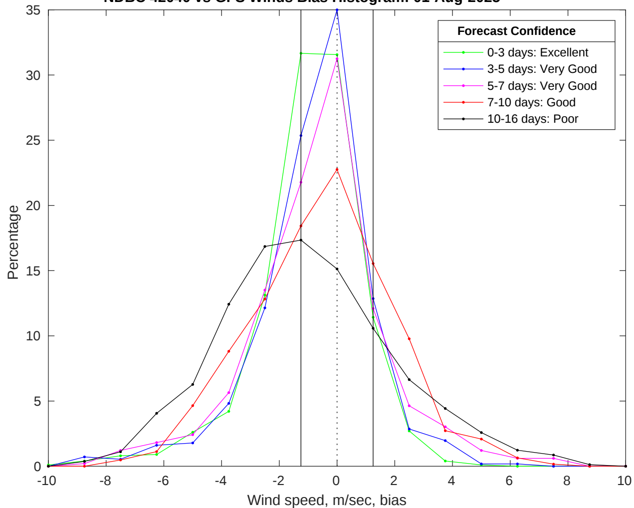
NDBC 42040 vs GFS Winds Bias Histogram: 01-Aug-2025
