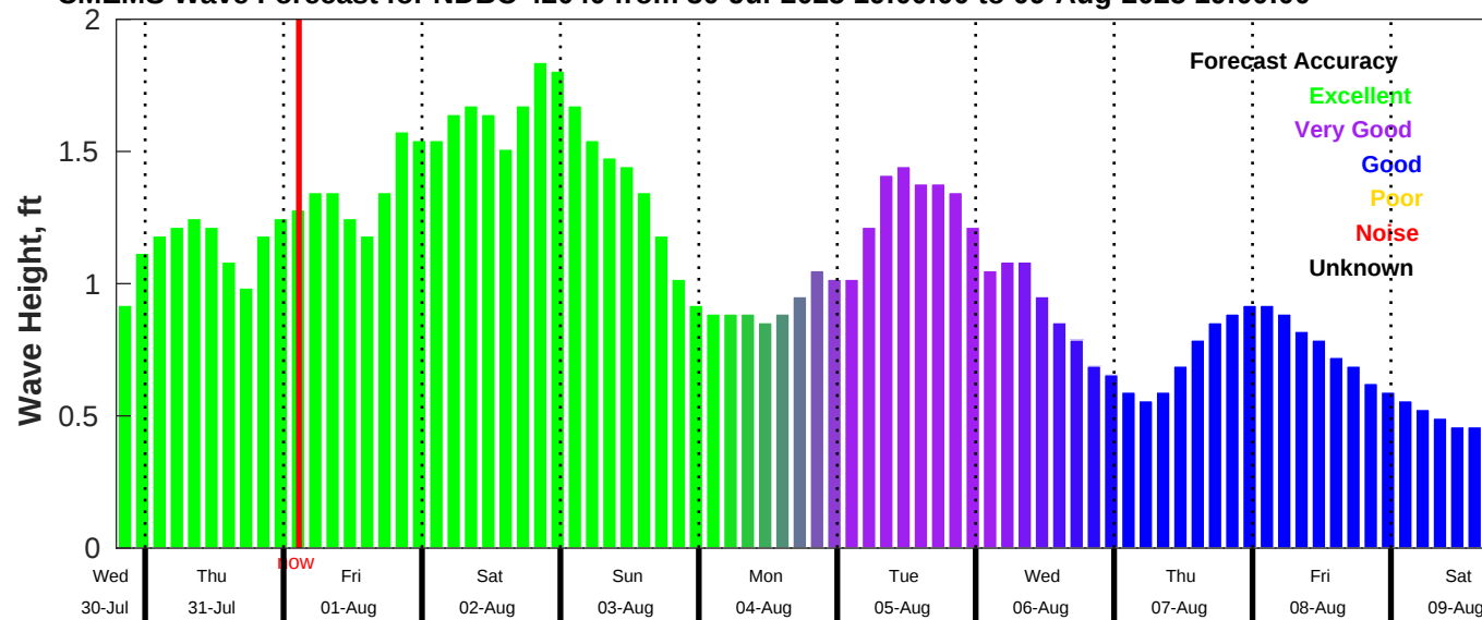
CMEMS Wave Forecast for NDBC 42040 from 30-Jul-2025 19:00:00 to 09-Aug-2025 19:00:00
