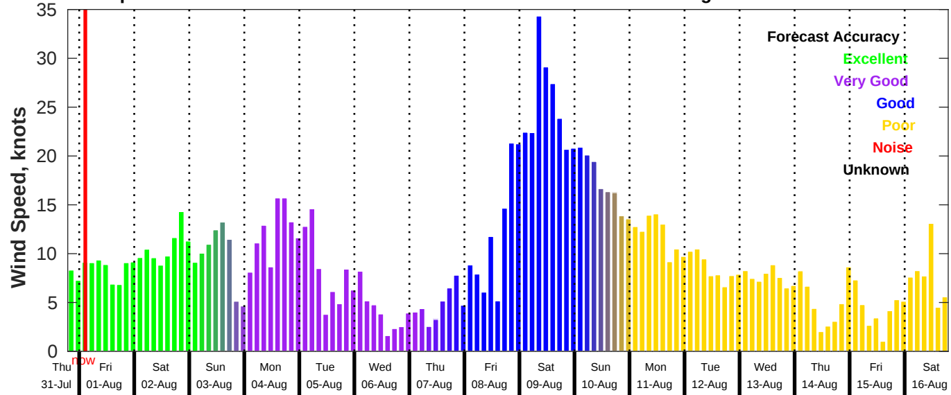
GFS Wind Speed Forecast for NDBC 42040 from 31-Jul-2025 19:00:00 to 16-Aug-2025 19:00:00
