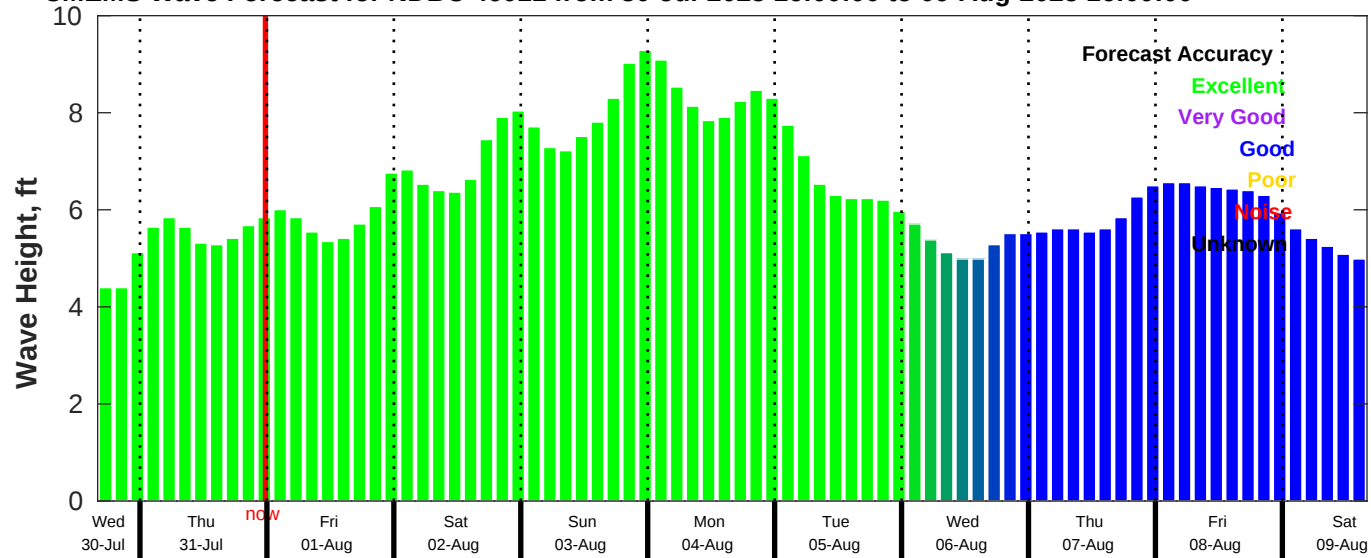
CMEMS Wave Forecast for NDBC 46011 from 30-Jul-2025 16:00:00 to 09-Aug-2025 16:00:00
