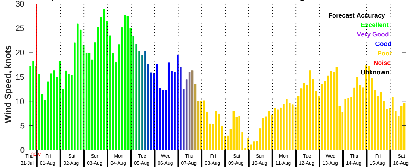
GFS Wind Speed Forecast for NDBC 46011 from 31-Jul-2025 16:00:00 to 16-Aug-2025 16:00:00
