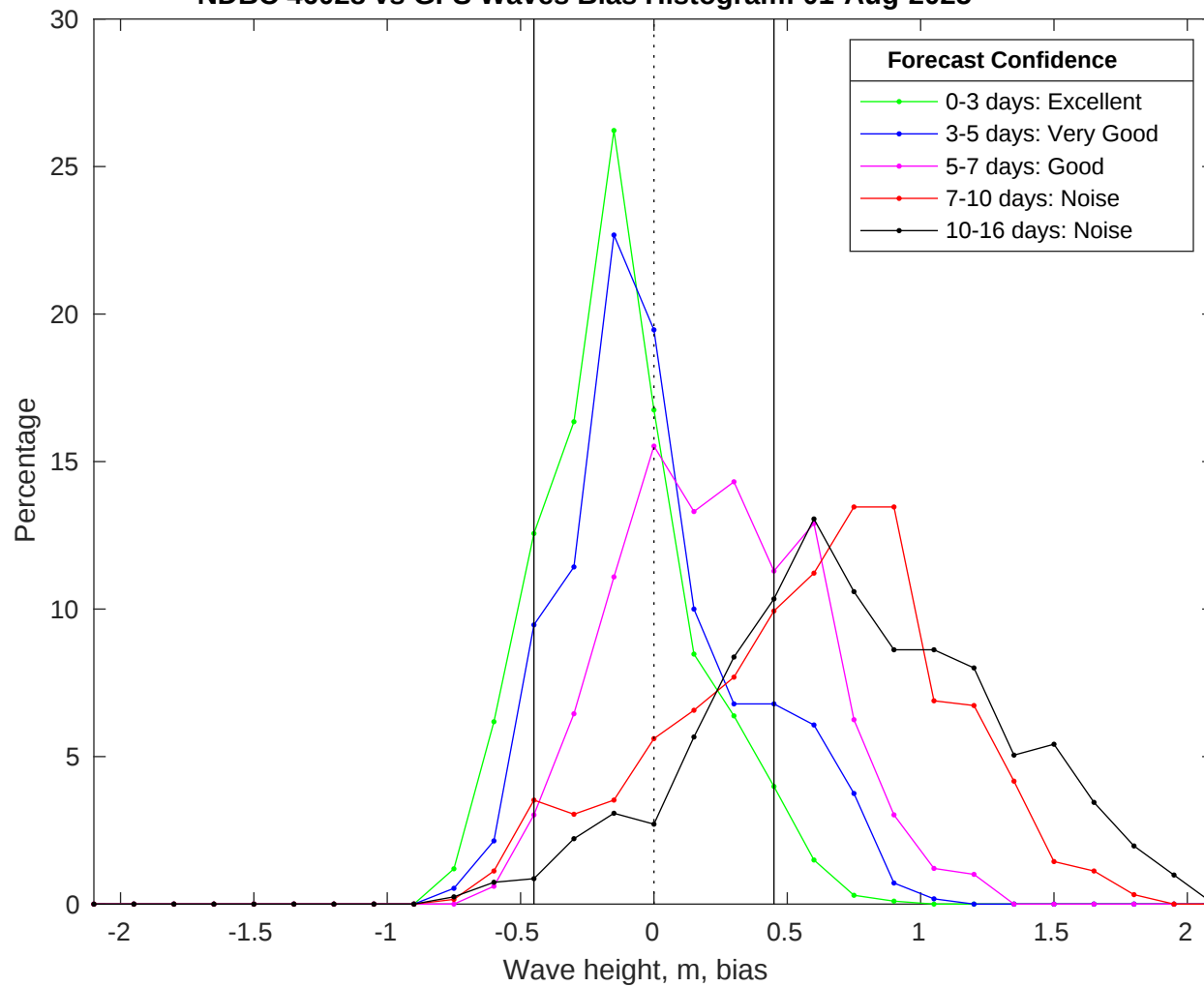
NDBC 46028 vs GFS Waves Bias Histogram: 01-Aug-2025
