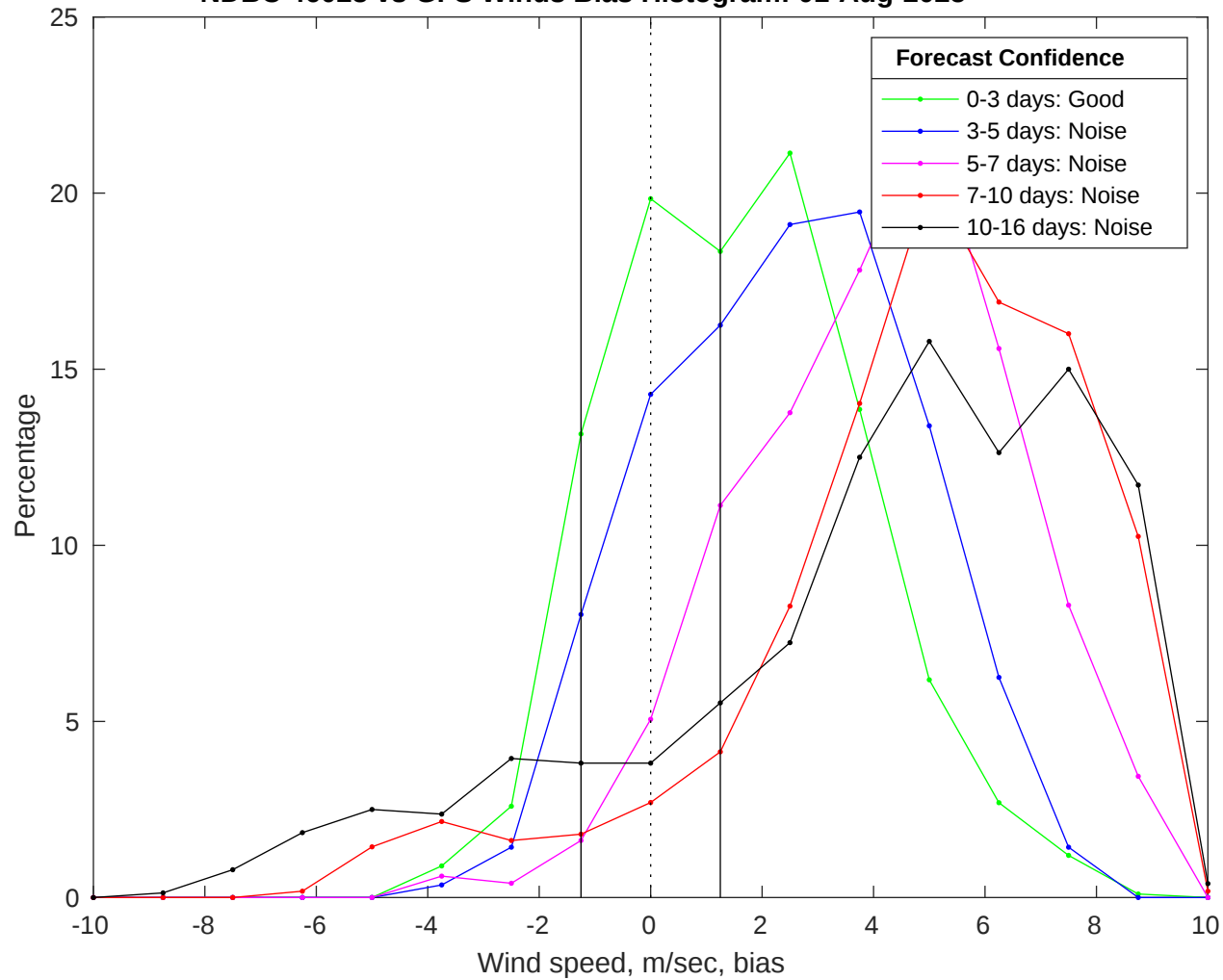
NDBC 46028 vs GFS Winds Bias Histogram: 01-Aug-2025
