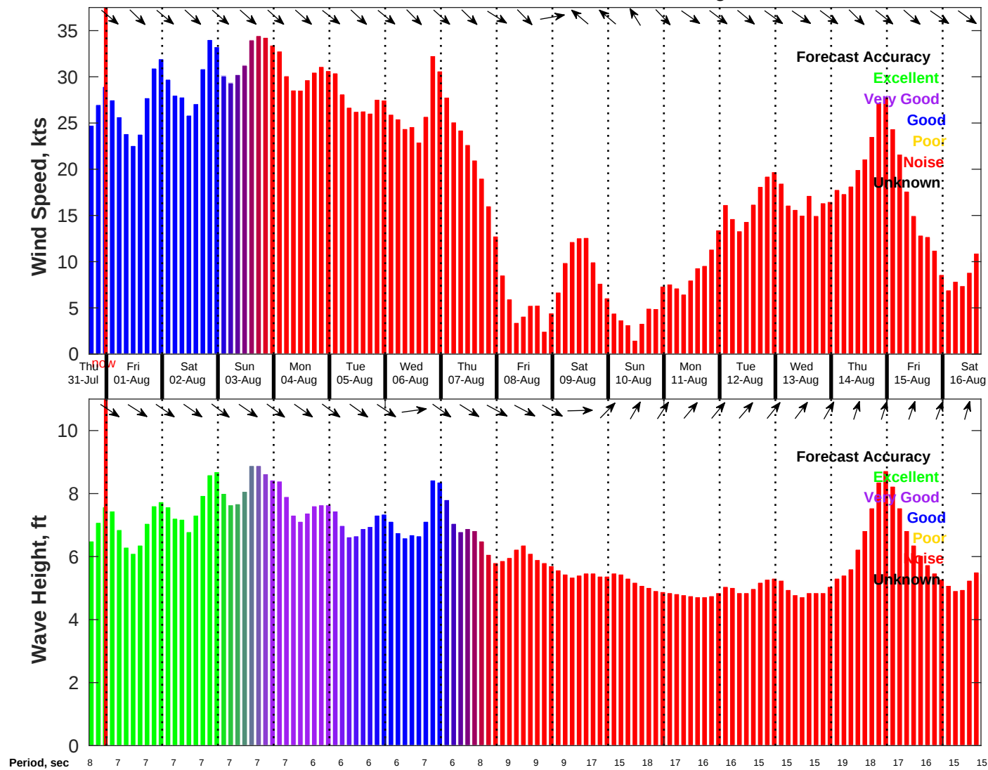
Wind & Wave Forecast for NDBC 46028 from 31-Jul-2025 16:00:00 to 16-Aug-2025 16:00:00
