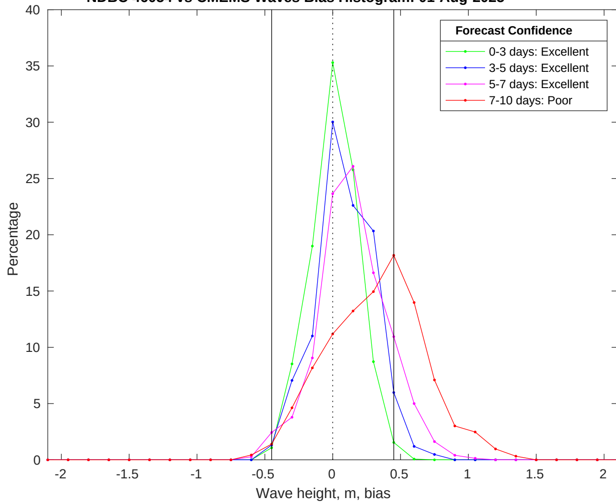
NDBC 46054 vs CMEMS Waves Bias Histogram: 01-Aug-2025
