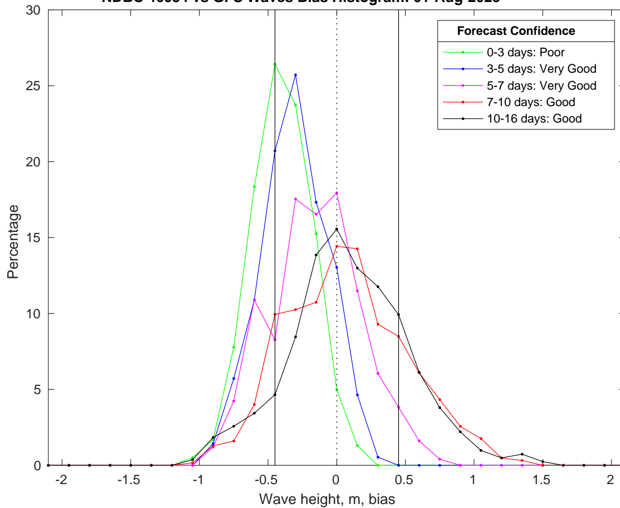
NDBC 46054 vs GFS Waves Bias Histogram: 01-Aug-2025
