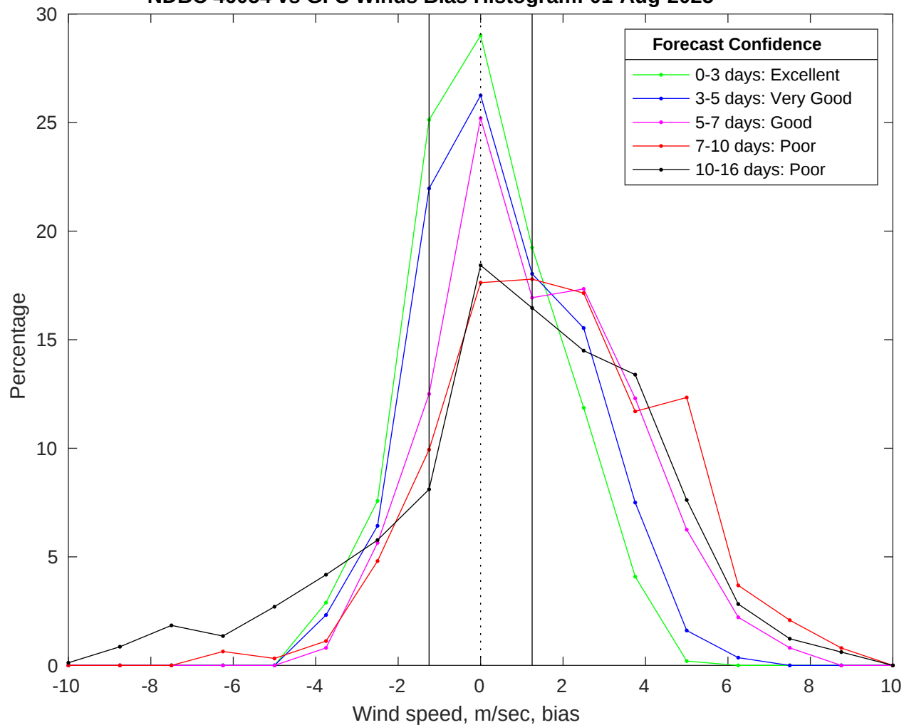
NDBC 46054 vs GFS Winds Bias Histogram: 01-Aug-2025
