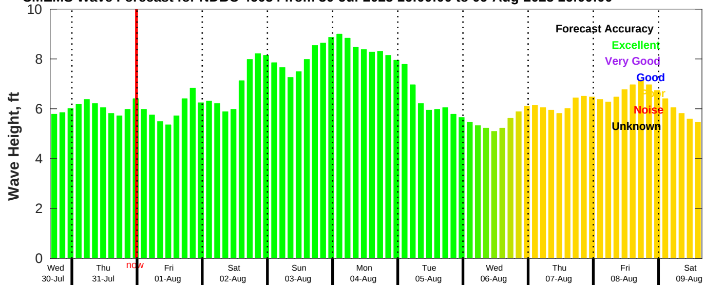
CMEMS Wave Forecast for NDBC 46054 from 30-Jul-2025 16:00:00 to 09-Aug-2025 16:00:00
