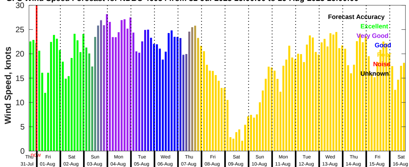
GFS Wind Speed Forecast for NDBC 46054 from 31-Jul-2025 16:00:00 to 16-Aug-2025 16:00:00
