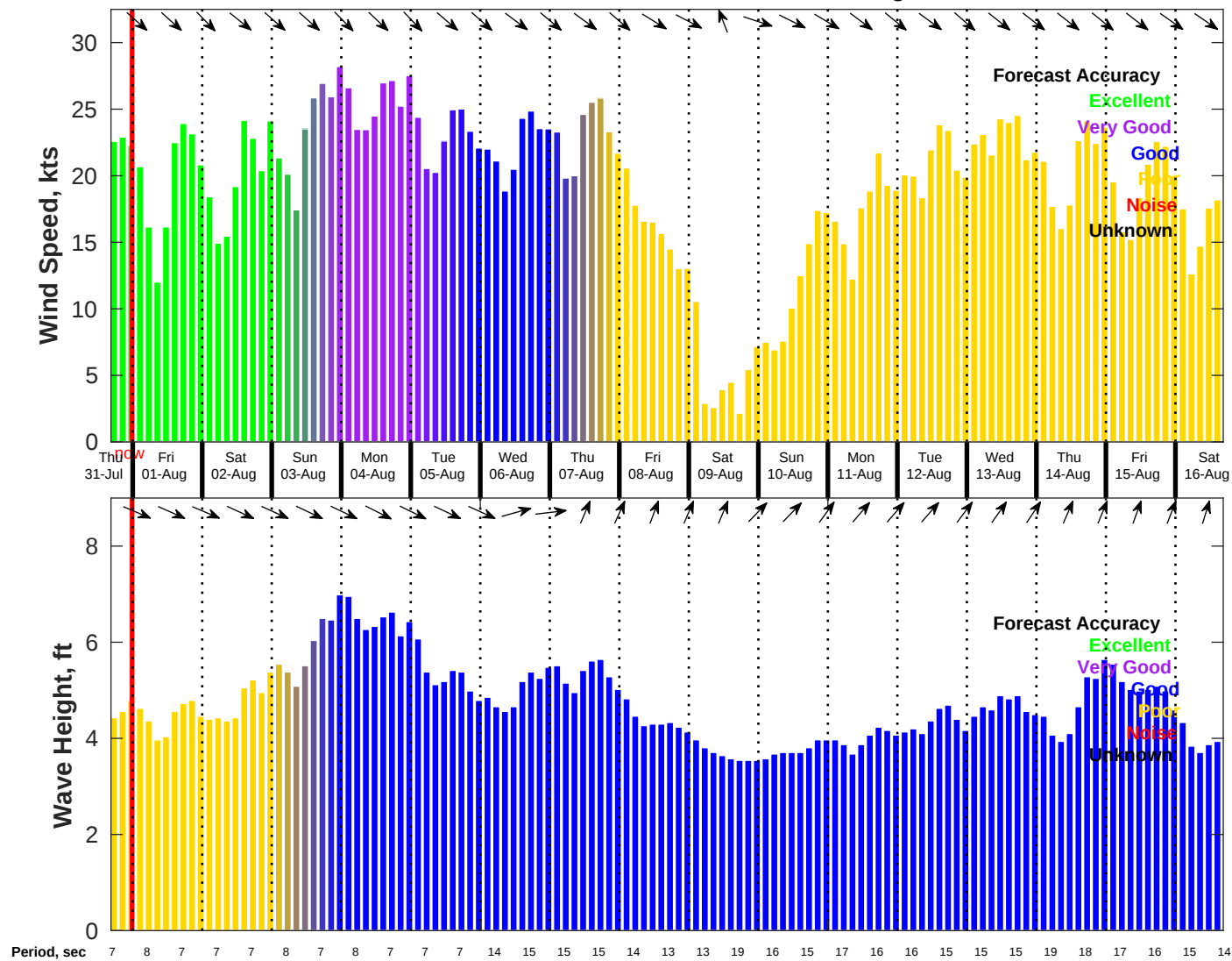
Wind & Wave Forecast for NDBC 46054 from 31-Jul-2025 16:00:00 to 16-Aug-2025 16:00:00
