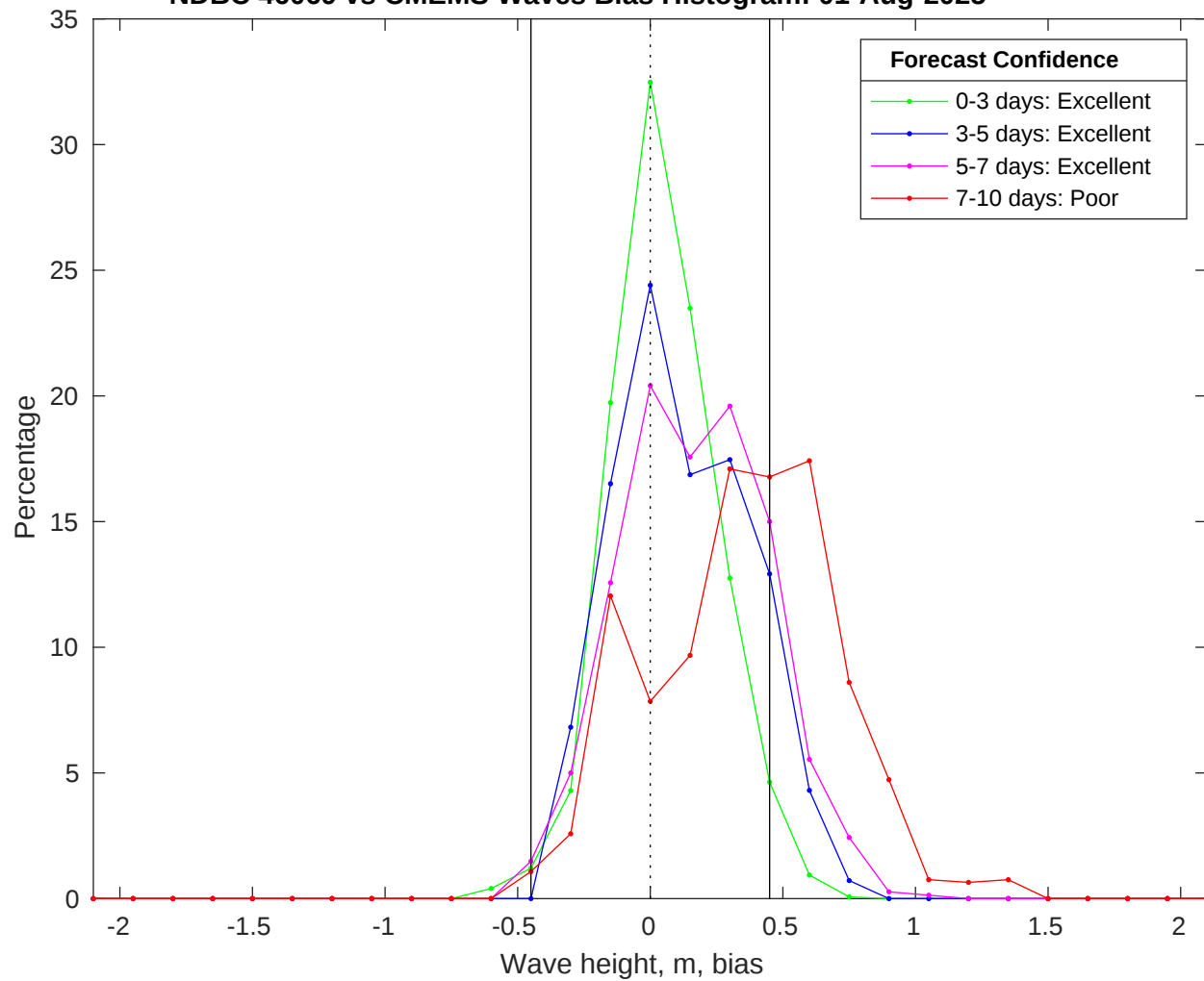
NDBC 46069 vs CMEMS Waves Bias Histogram: 01-Aug-2025
