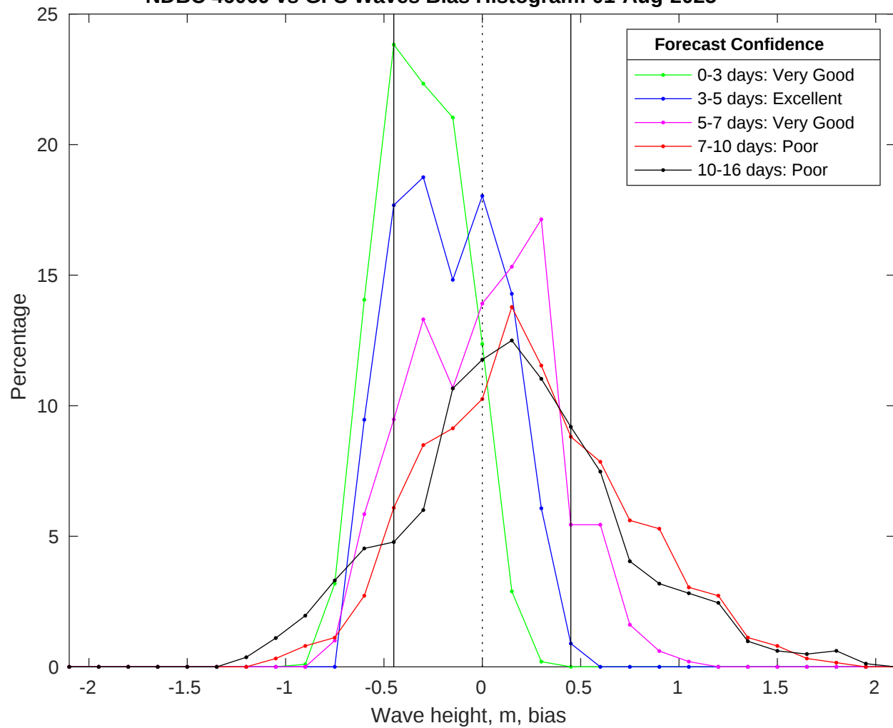
NDBC 46069 vs GFS Waves Bias Histogram: 01-Aug-2025
