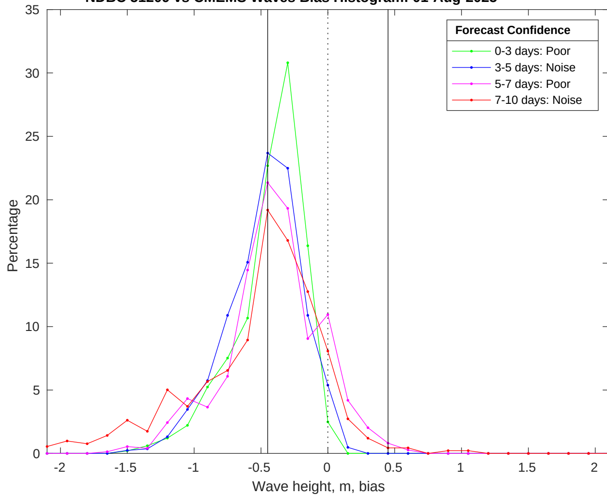
NDBC 51209 vs CMEMS Waves Bias Histogram: 01-Aug-2025
